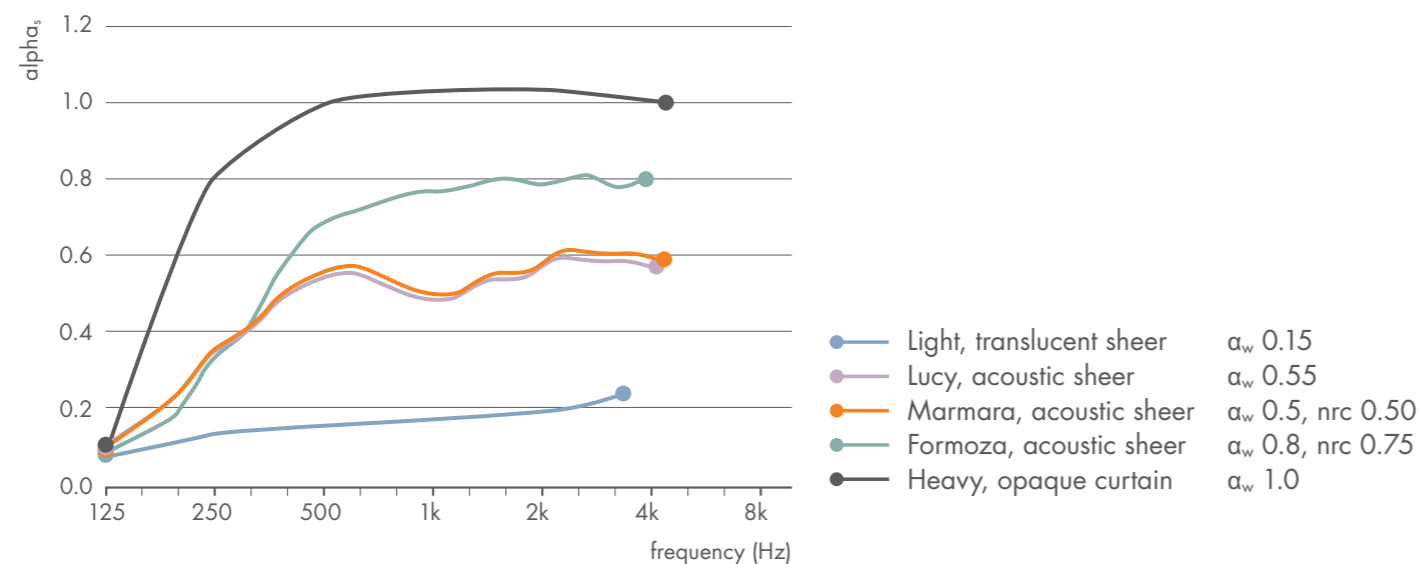
15 cm (6") gap between sheer and window or wall, fully pleated.
